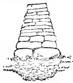
Fig. 5.—Cross Section of a well built wall.
